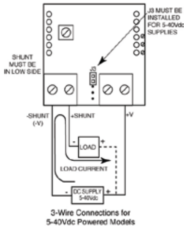
Low-Side Shunt Connections for 5-40Vdc Non-Isolated Supply Models
