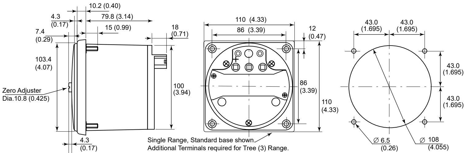
Fig. 1. HLS-110 Panel drilling plan. For instrument Dimensions.
